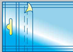
flat bag (recloseable) with euro hole punch or hole punch - from one film - (for dry and heavy products only)
